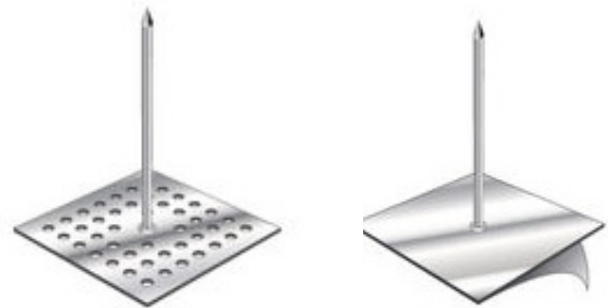
Insulation can also be held with perforated base hangers (uses adhesive) or with self adhering hangers.
