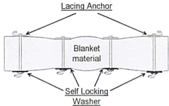
Lacing anchor & Quilting pins are used in the manufacturing of removeable blanket insulation.
